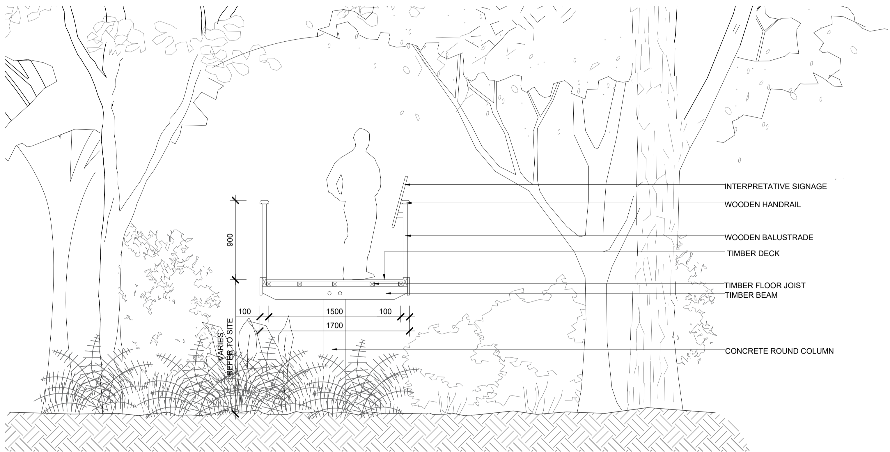
SECTION 1 SCALE 1:25 @ A1
