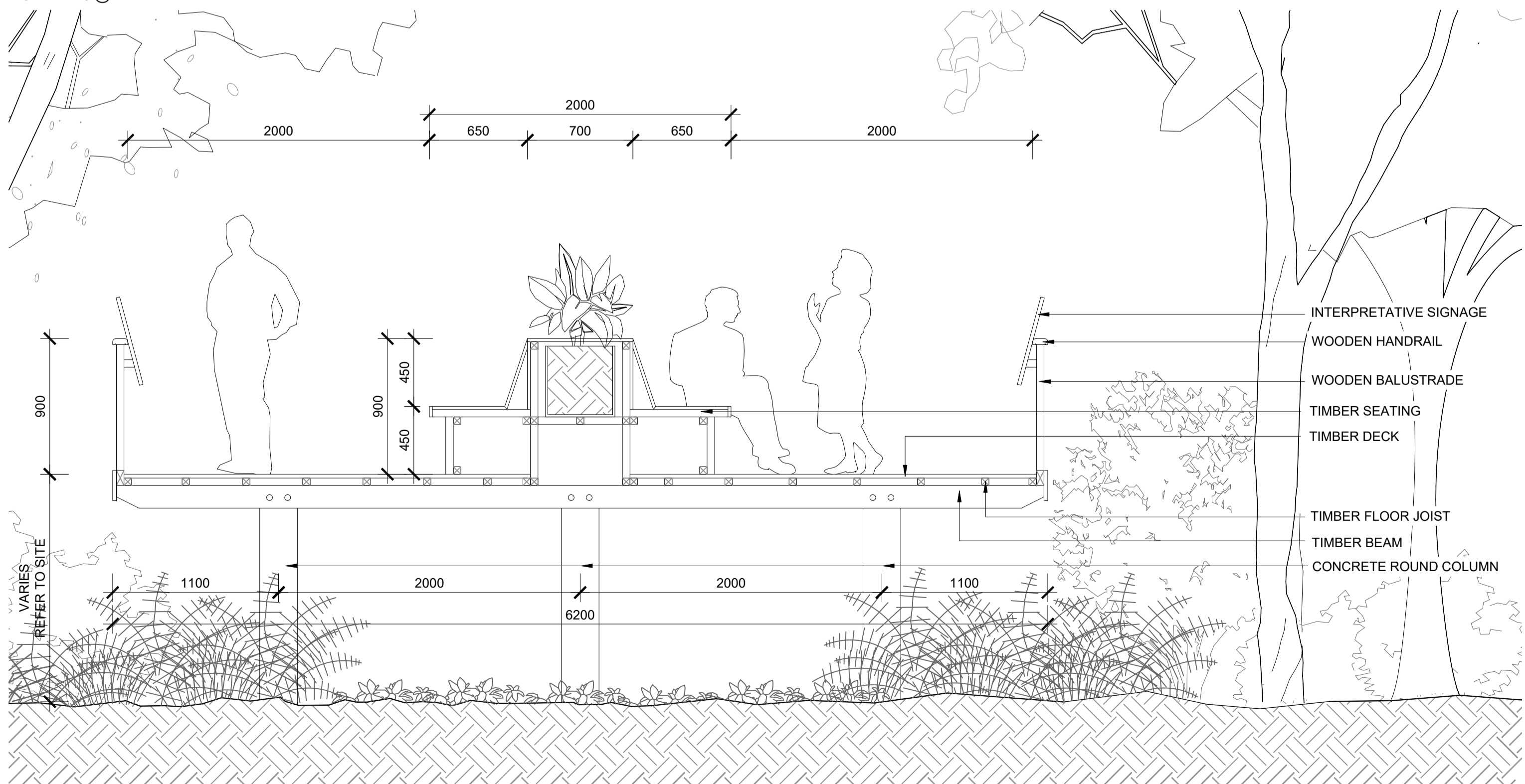
SECTION 2 SCALE 1:25 @ A1
