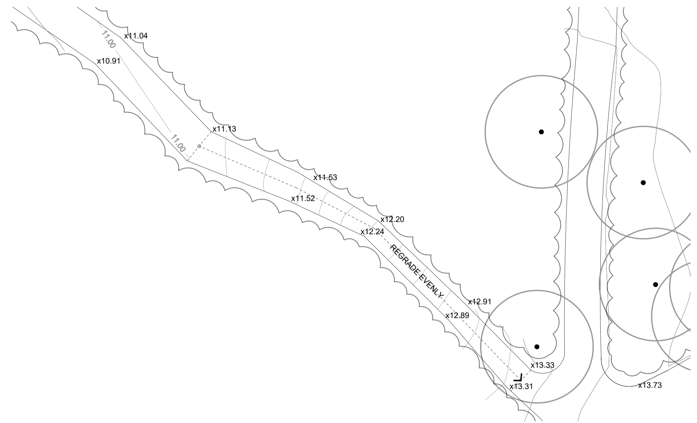
2 FOOTPATH RE-GRADING 2 (TOWARDS REPARIAN WALK) SCALE 1:100
